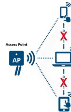
Fig. 8: Peer-to-Peer-Isolation
